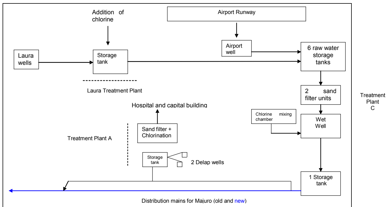
Figure 9 Schematic of Majuro reticulated water supply
